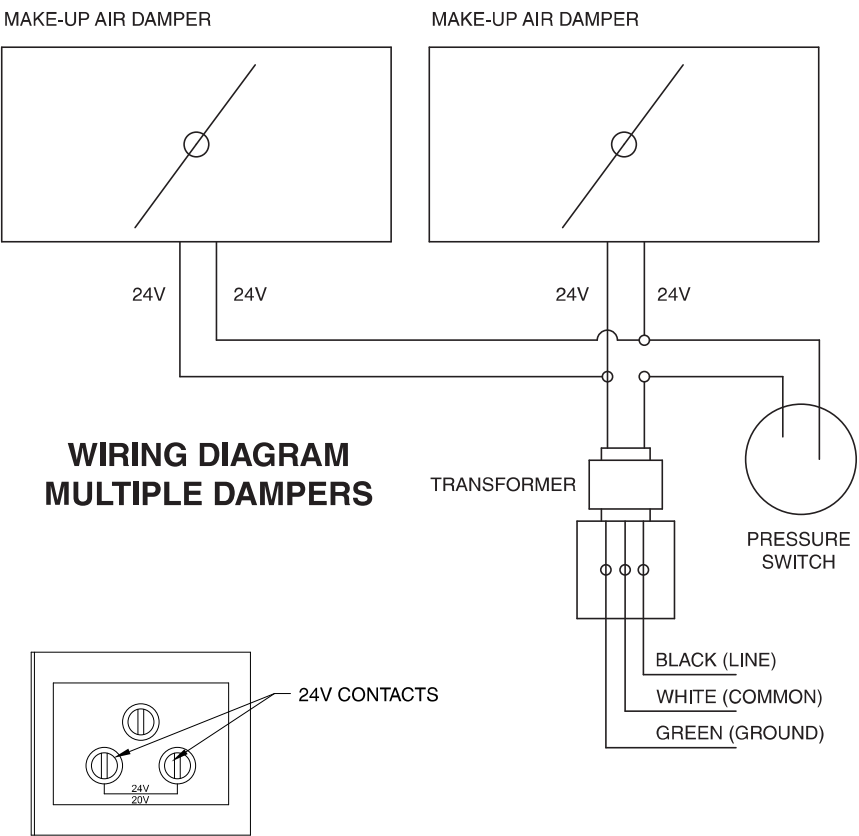
TRANSFORMER WIRING
