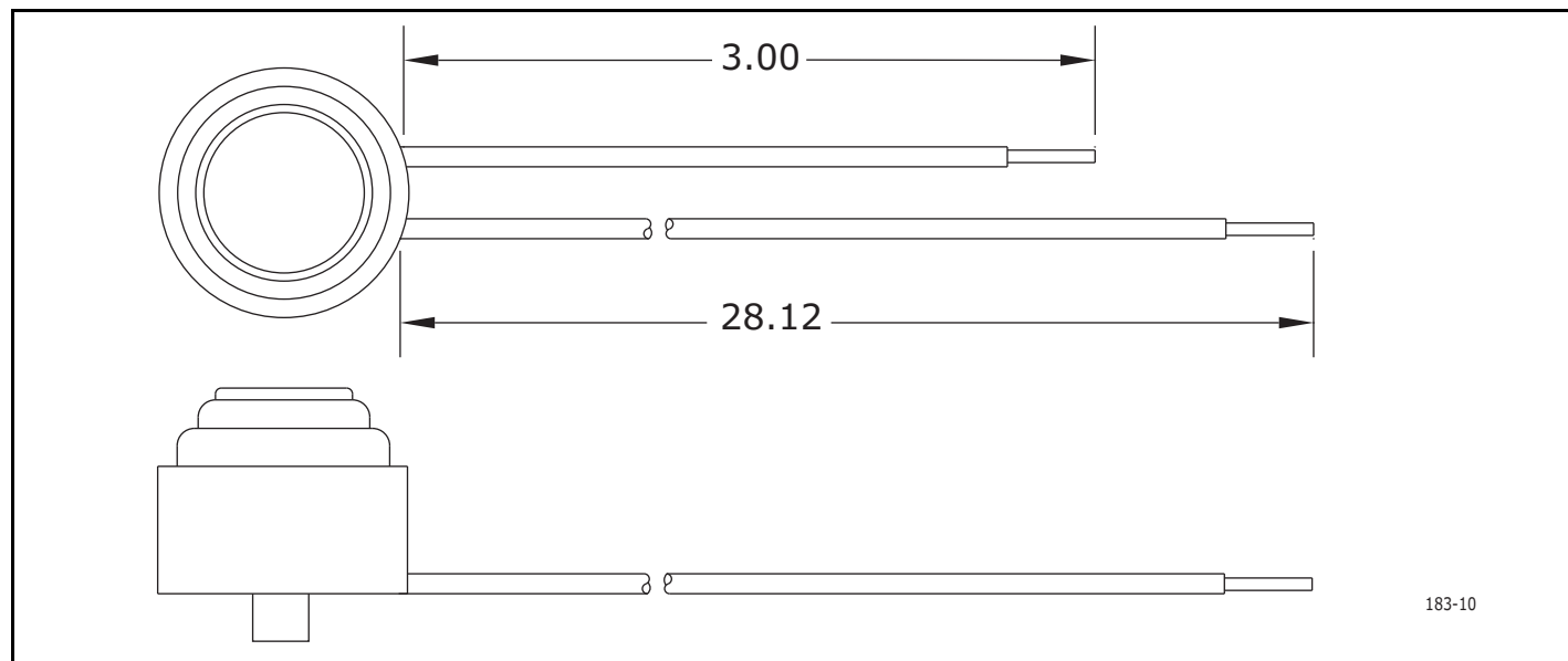
Figure 6. Limit Switch
