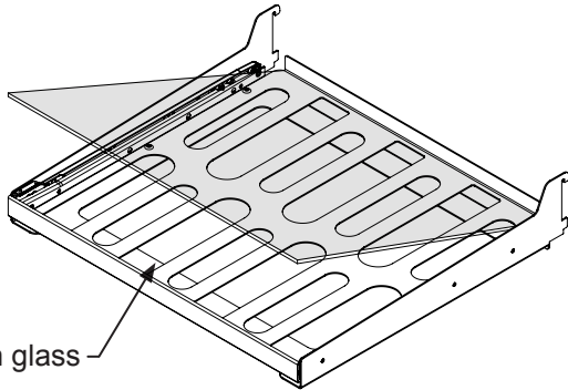
Figure 32 Wine cutout and flat glass shelf with vibration dampening mat, the glass can be removed for wine storage.
