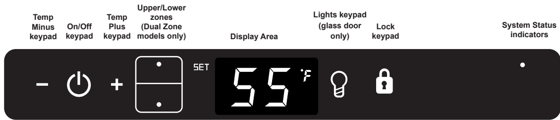
Figure 12 Electronic control
