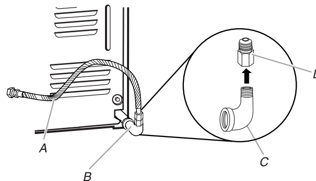
A. \frac{3}{8} " flexible gas connector
