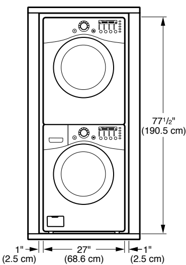
Required Dimensions for Installation With Stacking Kit
