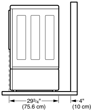
Required Dimensions for Installation With Pedestal
