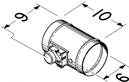
Model MD6S Model MD6TU
