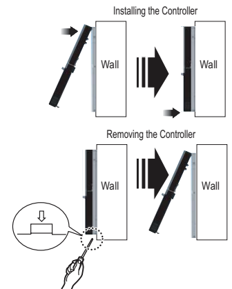
Figure 122: Installing / Removing the Controller.
