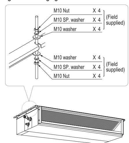
Figure 108: Hanging the Indoor Unit.
