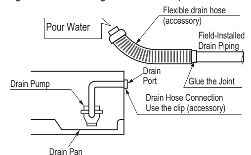
Figure 177: Checking the Drain Pump.
