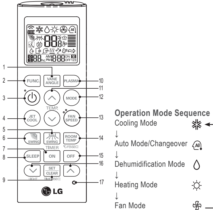
Figure 182:AKB73757604 Wireless Handheld Controller.
