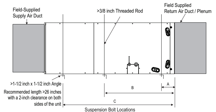
Figure 201: Horizontal Installation.
