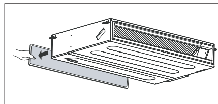
Figure 113: Checking the Drainage System.
