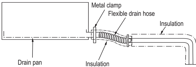
Figure 258: Diagram of an Indoor Unit with a Gravity Drain.
