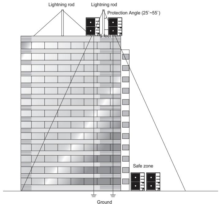
Figure 257: Lightning Protection Diagram.
