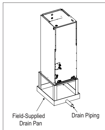
Figure 203: Vertical Installation Drain System.
