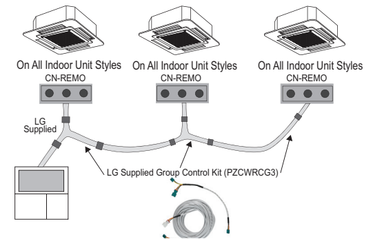
Figure 272: Example of Indoor Unit Group to Zone Controller Connections (CN-REMO).
