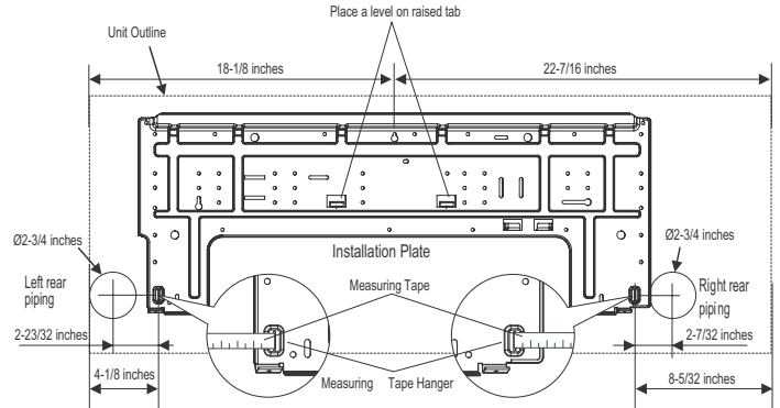
Figure 12: Installation Plate for LAN180HSV5 Units.
