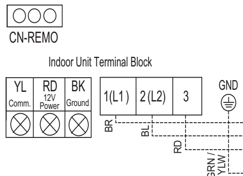
Figure 149: Wired Controller Connections on the Indoor Unit Terminal Block.
