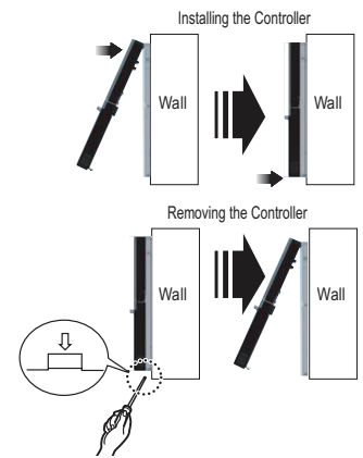
Figure 93: Installing / Removing the Controller.
