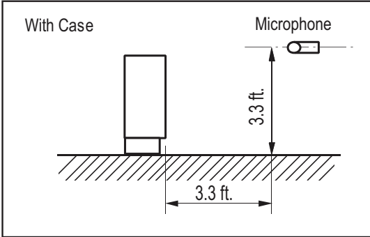
Figure 224: Sound Pressure Level Measurement Location.
