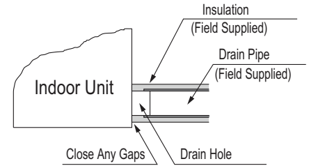
Figure 109: Drain Connection.
