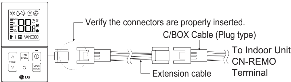
Figure 213:PZCWRC1 LG Wired Remote Extension Cable.
