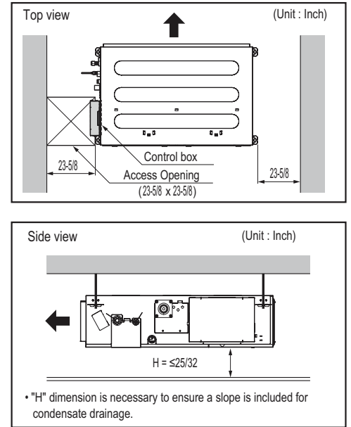
Figure 102: General Installation Guidelines.
