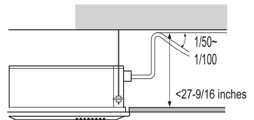
Figure 176: Indoor Unit Drain Piping.
