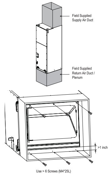
Figure 200: Vertical Installation / Attaching the Bottom Duct.
