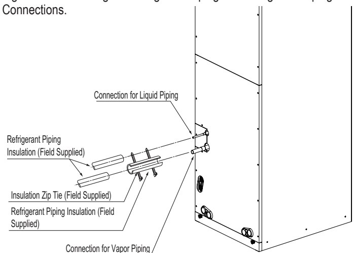
Figure 244: Insulating the Refrigerant Piping and Refrigerant Piping Connections.
