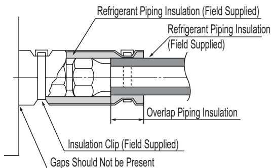
Figure 209: Close Up of Refrigerant Piping Connection Insulation.
