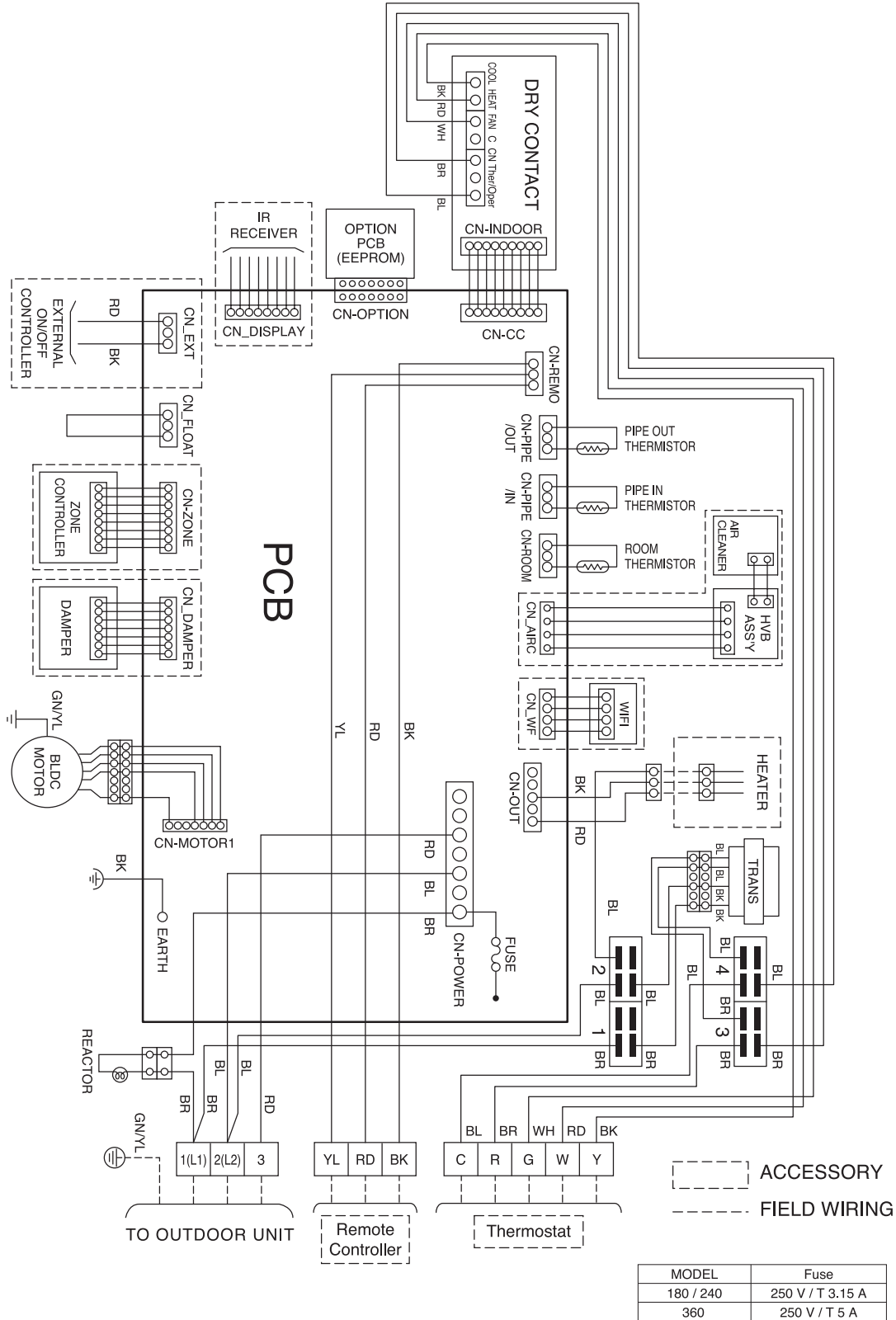
Figure 228: Four-way Vertical-Horizontal Air-Handling Indoor Unit Wiring Diagram.
