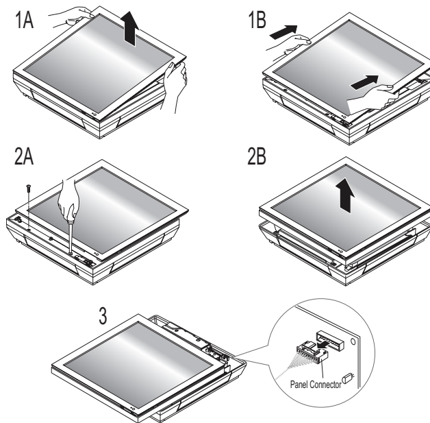
Figure 40: Preparing for Installation.
