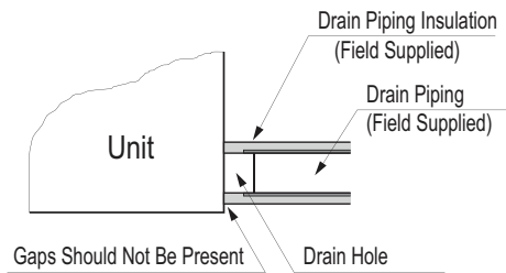
Figure 239: Close up of Drain Piping Connection.
