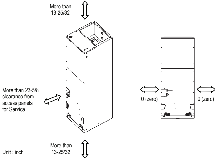
Figure 229: Clearance Requirements.
