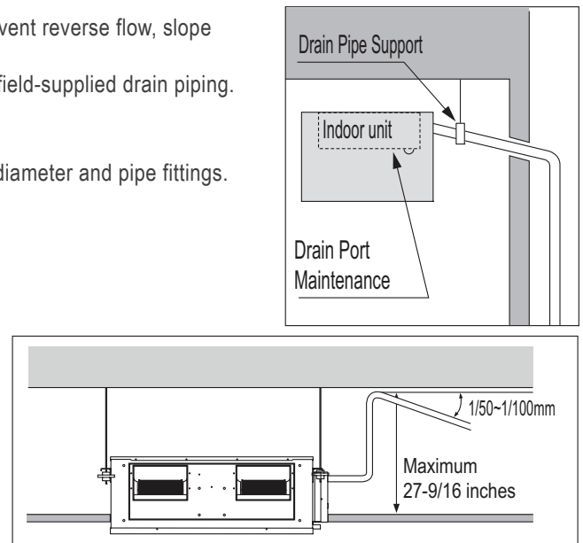
Figure 139: Indoor Unit Drain Piping.
