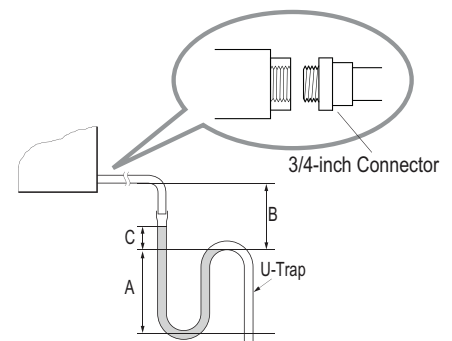
Figure 240: Installing the U-Trap.
