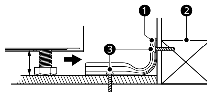
1 Anti-tip Bracket
