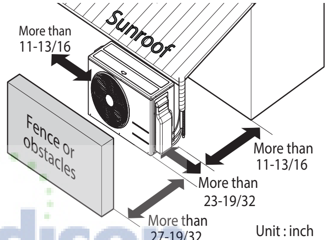
Figure 28: Outdoor Unit Sunroof/Awning Clearances
