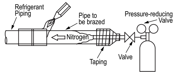
Figure 40: Refrigerant Pipe Brazing.
