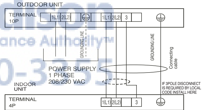
Figure 46: Terminal Block Wiring Diagram - LSU240HLV, LSU300HLV, LSU360HLV
