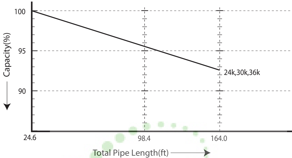
Figure 22: LS240HLV, LS300HLV, LS360HLV Heating Coefficient Factor Heating
