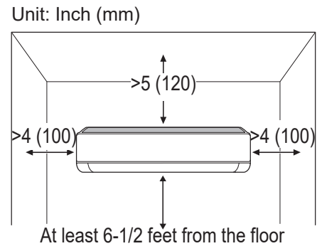
Figure 19: Extended Piping Wall-Mounted Indoor Unit Clearance Requirements.
