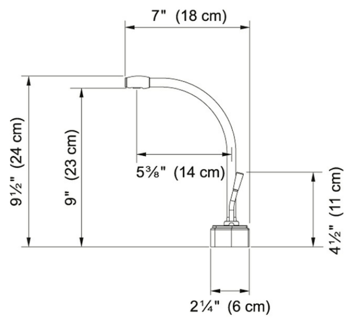
Technical Drawing
