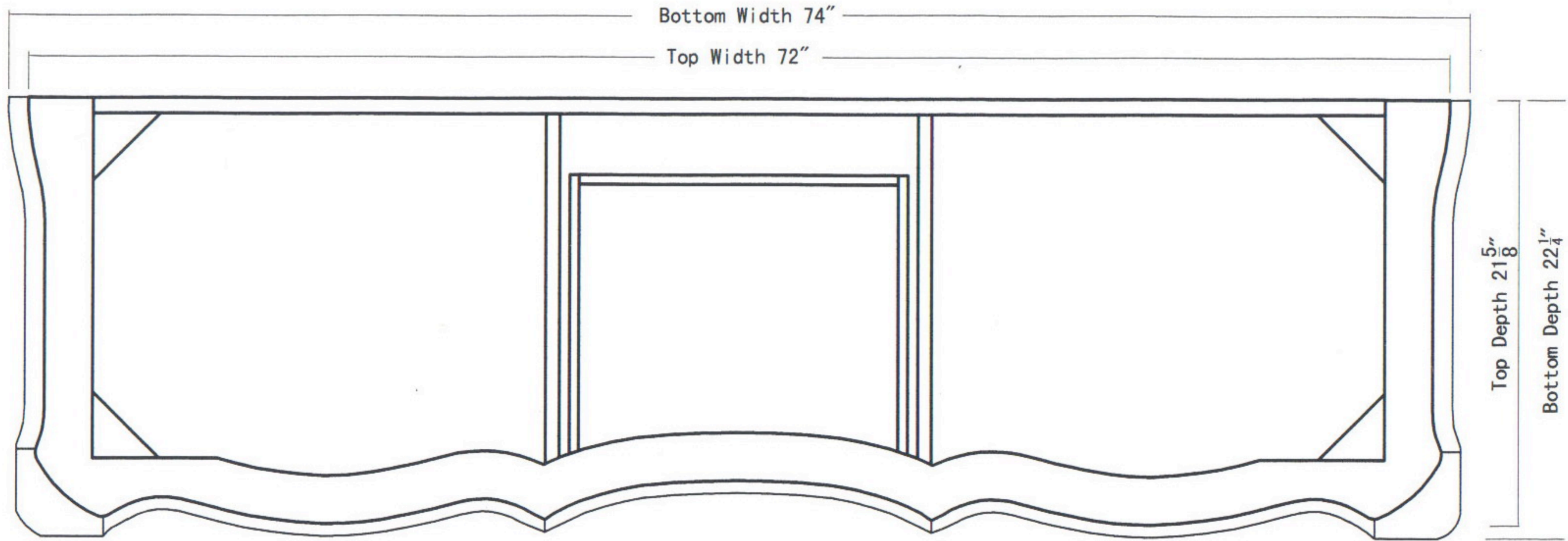
TOP VIEW
