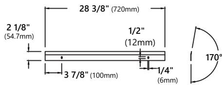
Mounting Plate
