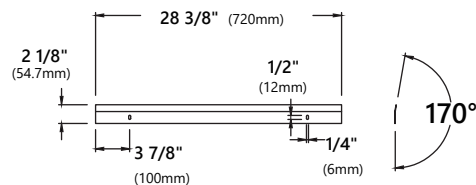
Mounting Plate
