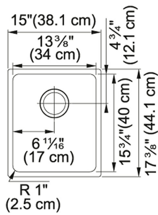
Technical Drawing
