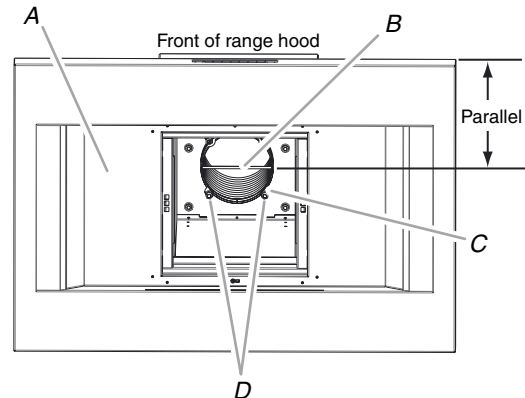
A. Inside of range hood cavity B. Mounting boss handle C. Half slots in module top cover (4) D. Nuts (4)
