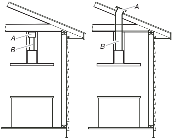
A. Deflector B. 6" (15.2 cm) round vent A. Roof cap B. 6" (15.2 cm) round vent
