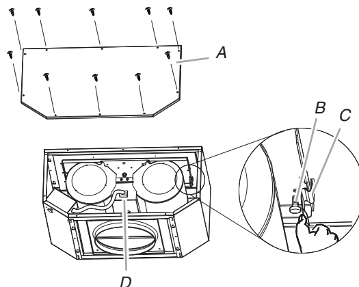
A. Front cover B. Blower mounting screws C. Spring clip D. Motor electrical plug
