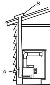
A. 6" (15.2 cm) round ducting transitioned to 3 \frac{1}{4} " x 10" (8.3 cm x 25.4 cm) rectangular floor venting B. Roof cap
