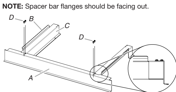
A. Bottom vent B. Spacer bar flange C. Spacer bars D. \frac{3}{8} " hex-head washer screws
