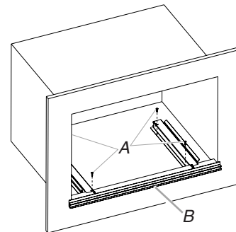
A. \frac{3}{4} " flat-head screws B. Spacer kit assembly
