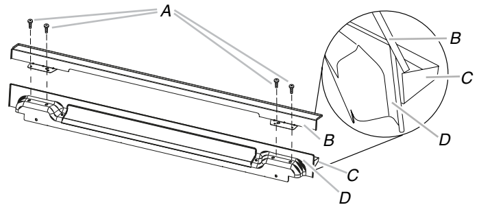
A. #8-18 x 1/4" screws B. Deflector bracket
