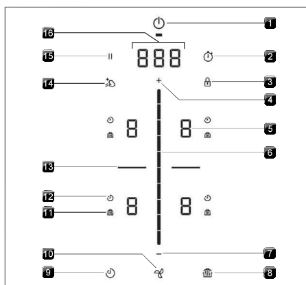
Fig. 6.3 Operating panel
