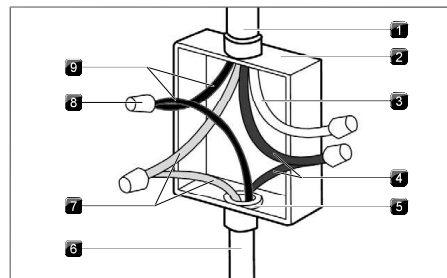
Fig. 11.20 4-Wire Cable
