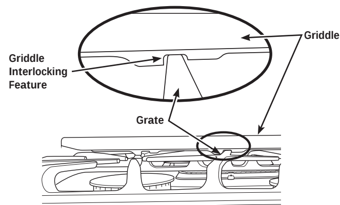
Side View: Properly positioned Removable Nonstick Griddle.
