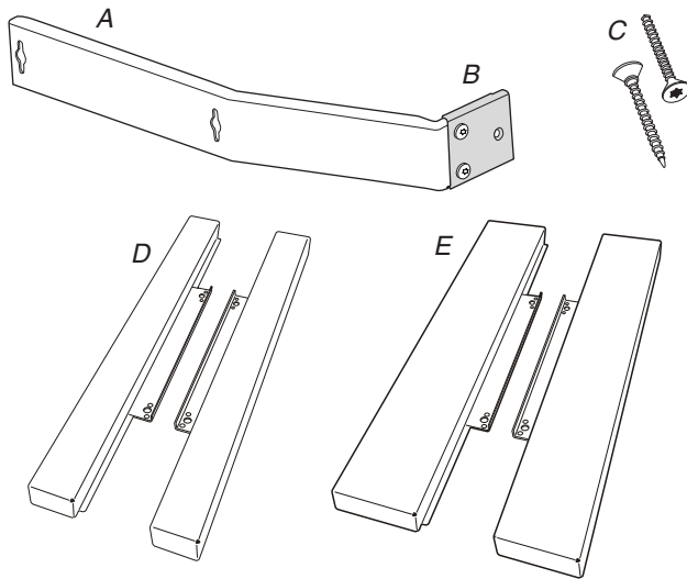
A. Side brackets (2) B. Removable extension plates (shaded piece, 2)
