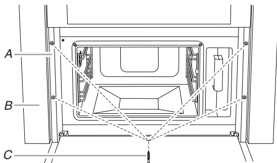
A. Door facing frame B. Trim panel C. 1" T10 screws (4)
