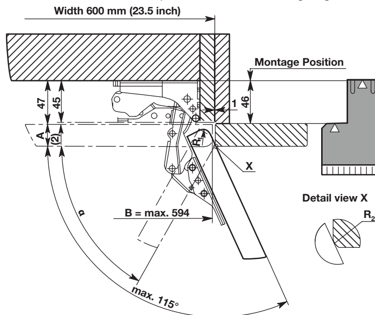
Cabinet frame wall thickness 16 mm
