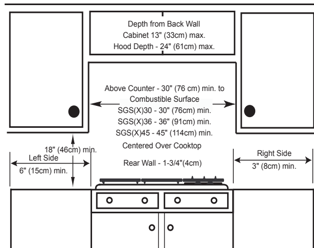
Figure 1 - Installed Dimensions (from cooktop edges)
