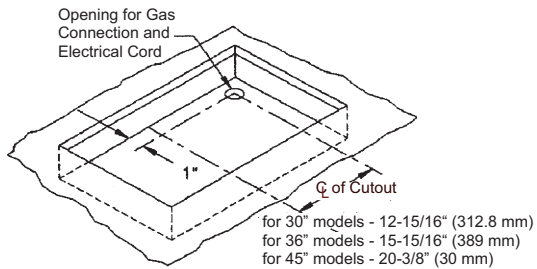
Figure 5 - Rough-in Box Area
