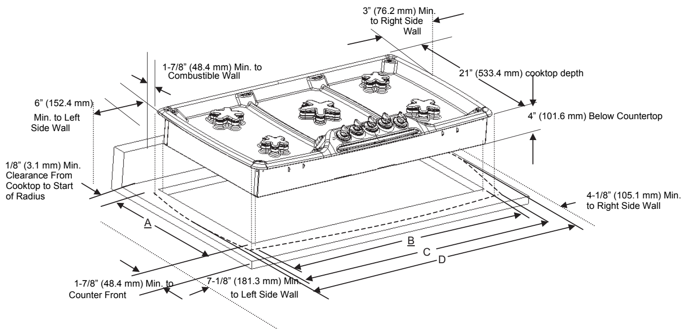
Figure 2 - Cutout Dimensions
