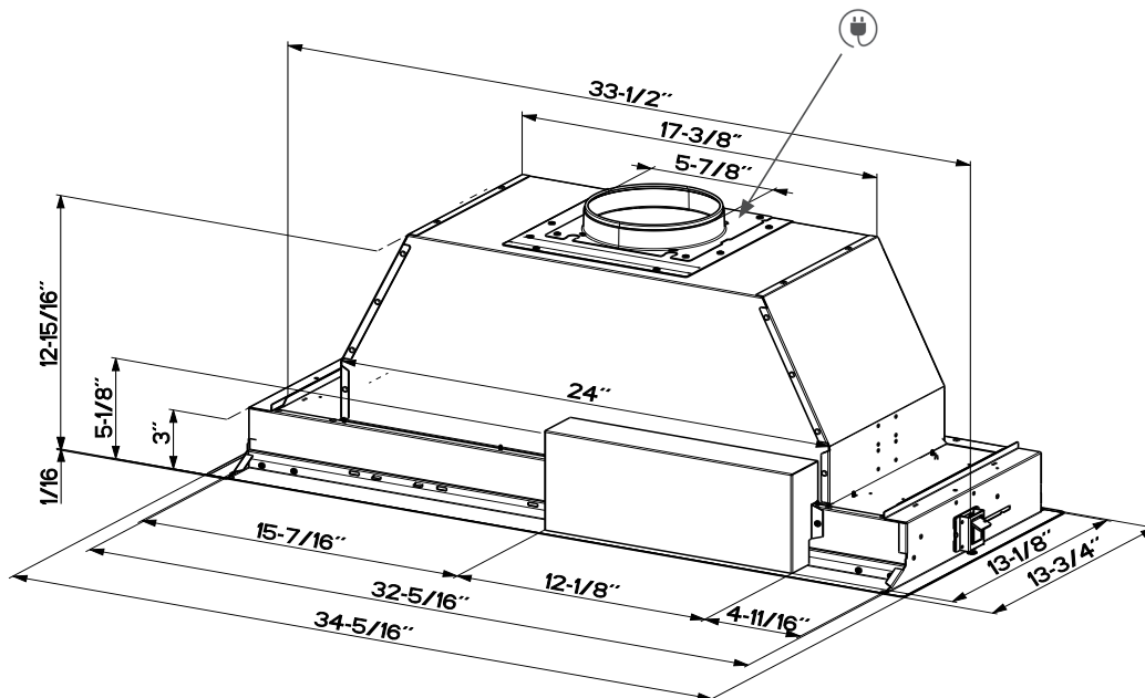
35" FRONT VIEW
