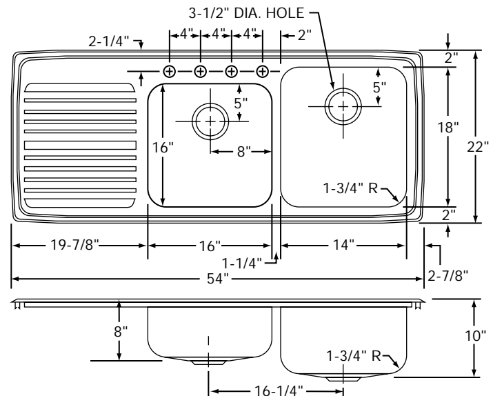
Model ILGR5422R4 Illustrated
