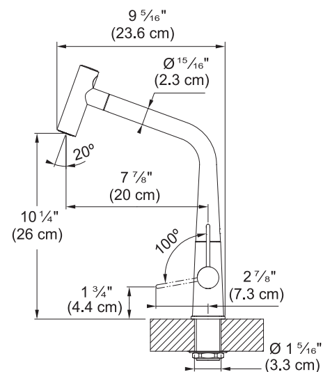
Dimensional Drawing
