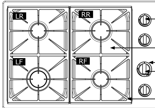
DYCT304G: Top View
