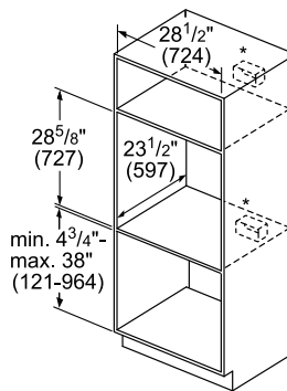
30" Speed Oven Over Storage / Warming Drawer
