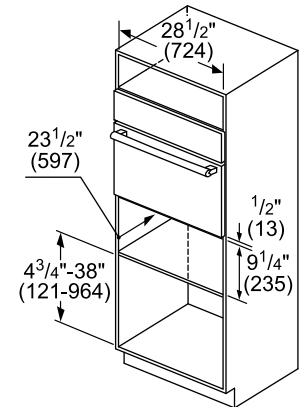
30" Storage / Warming Drawer Wall-Mounted
