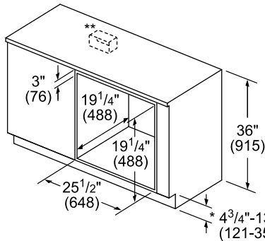
Under-counter Installation
