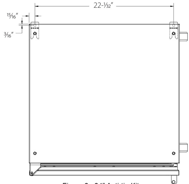
Figure 2. 24" Anti-tip Kit
