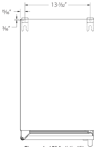
Figure 1. 15" Anti-tip Kit
