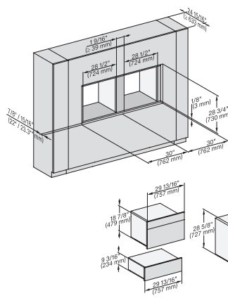
H 6x80 BP, H 6x70 BM, ESW 6x85, H 6x80-2BP, H7x70BM/BMX, ESW 7x70, EVS 7670, Installation drawing, Flush inset, NA
