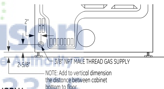
DRYER GAS SUPPLY CONNECTION
