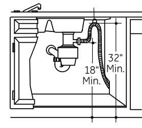
Disposer Installation
