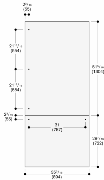
Niche width 35.5" (900 mm)
