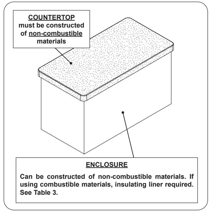
Fig. 9-1 Enclosure detail
