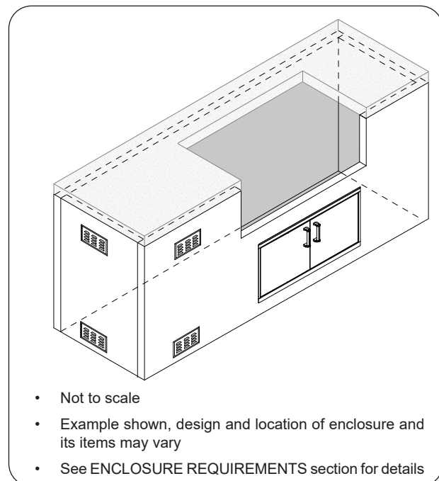
Fig. 23-1 Enclosure construction overview
