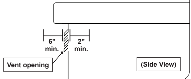
Fig. 8-2 Vent openings clearance
