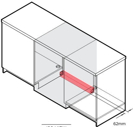
ISO VIEW
