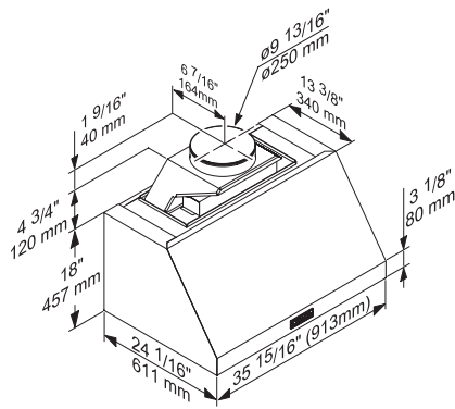
DAR1230 (installation drawing)
