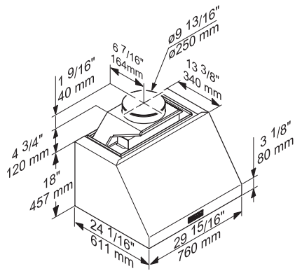
DAR1220 (Installation drawing)
