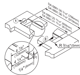
DA 6881, DA 6891 Downdraft (Installation drawing)
