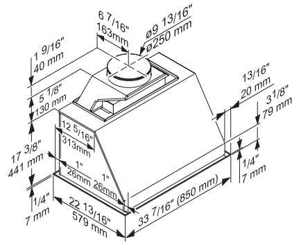
DAR1130 (installation drawing)
