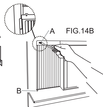
A. #10 X 1/2" round-head screw B. Slotted hole in the bottom of the curtain
