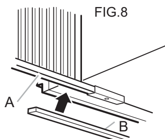
A. Curtain housing B. Foam adhesive seal
