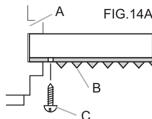
A. Window channel B. left-hand curtain C. #10 X 1/2" round-head screw
