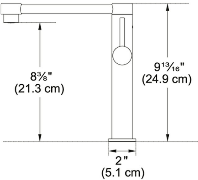
Technical Drawing
