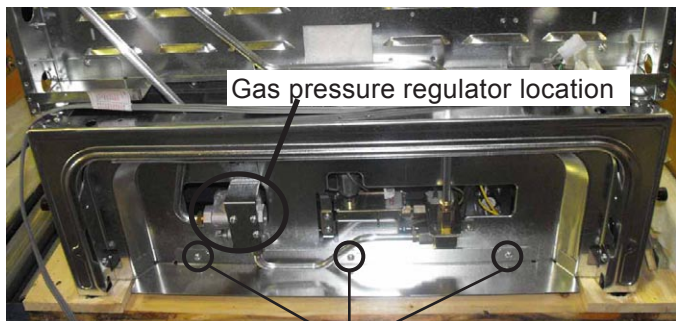
To remove the line protector, remove the 3 screws.
