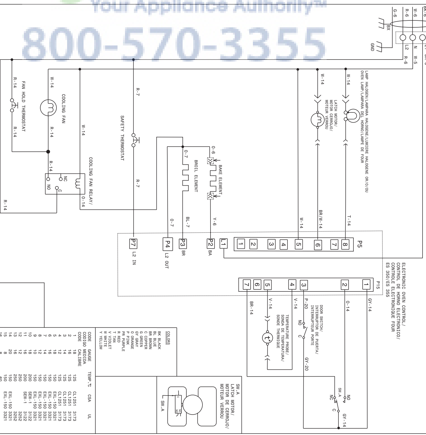
OVEN CIRCUIT//CIRCUITO DE HORNO//CIRCUIT FOUR
