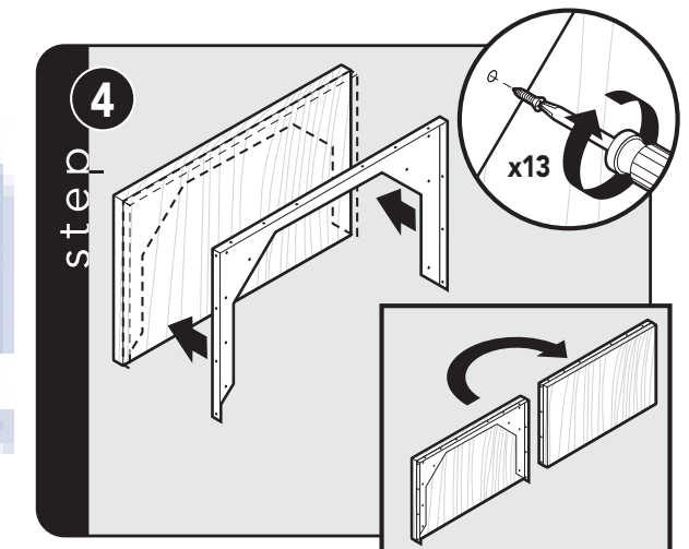
Attach bracket to the custom panel.
