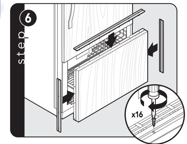
Reinstall door trim and door trim screws.
