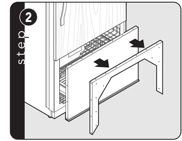
Remove bracket.
