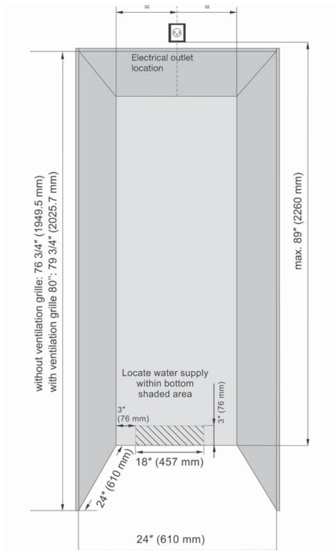
Fig. 6 Single installation
