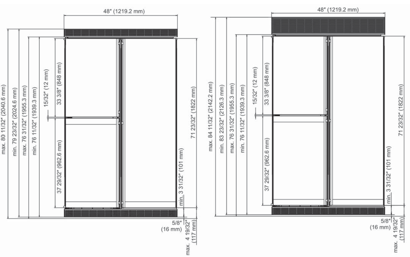
Fig. 4 Side-by-side installation: SBS 246 and SBS 241 with 80" or 84" ventilation grille
