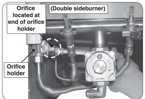
Fig. 30-4 Double sideburner orifice locations
