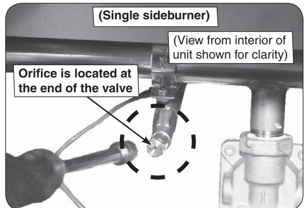
Fig. 30-3 Single sideburner orifice location
