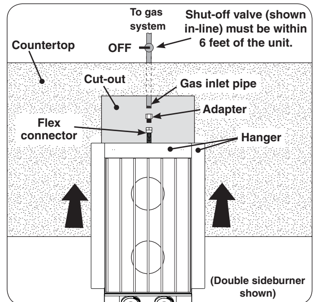
Fig. 19-4 Household propane & natural gas diagram
