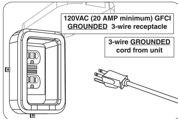
Fig. 21-2 Connect power cord
