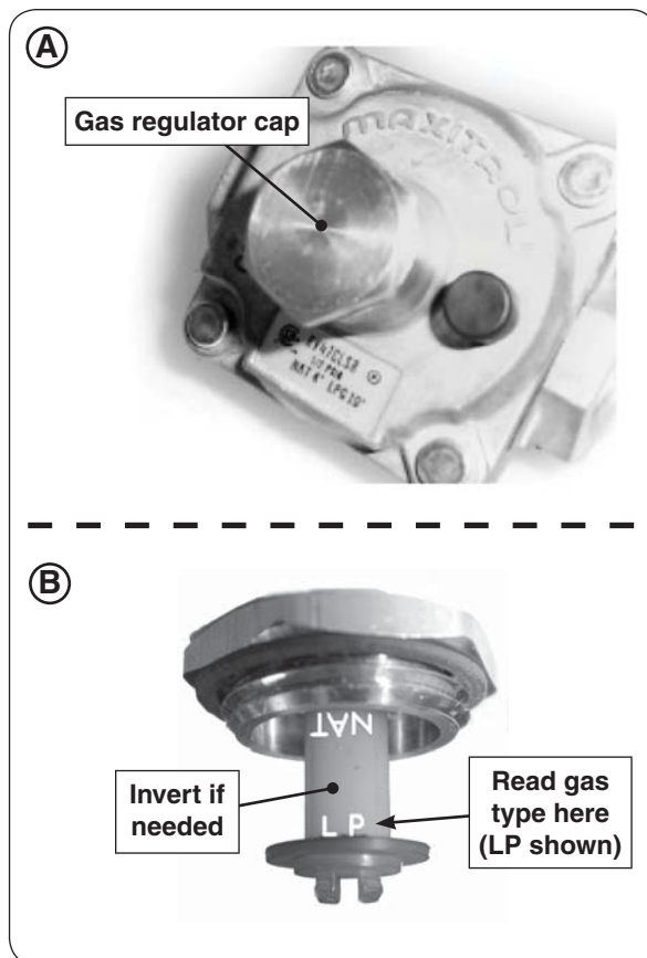
Fig. 29-1 Convert regulator
